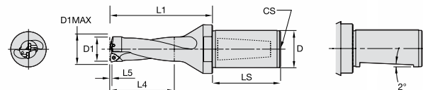
Drill FIX DFT Bodies
