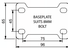
75 -125MM RIGID CASTOR
