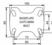
RIGID CASTOR
