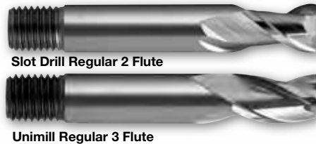
Unimill Regular 3 Flute
