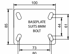
SWIVEL CASTOR
